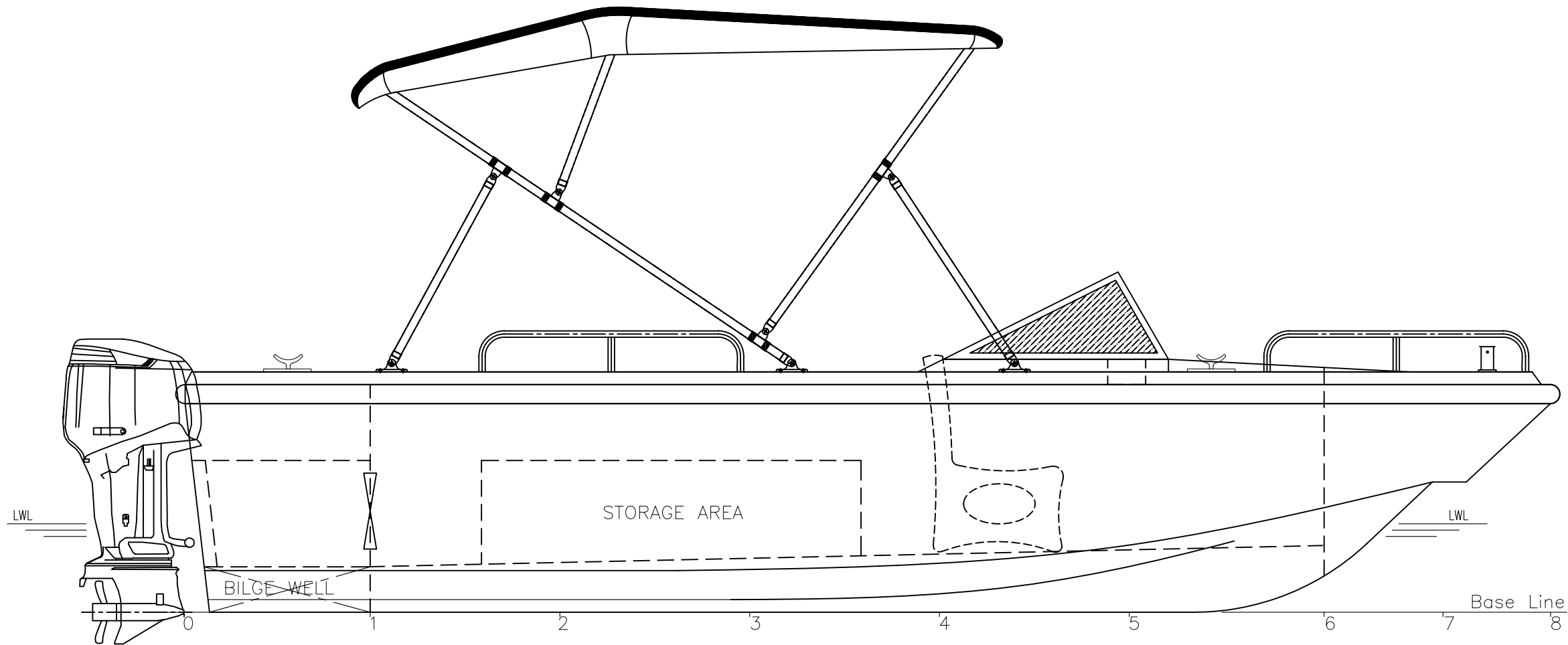
PROFILE VIEW
