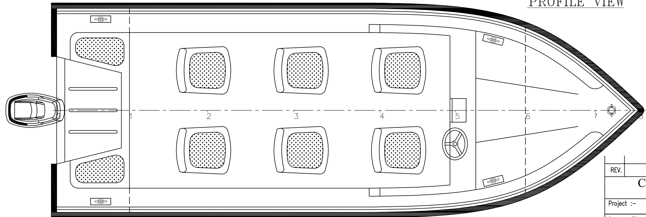
PLAN VIEW
