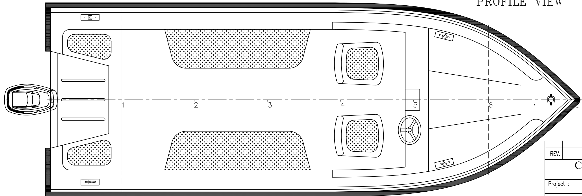
PLAN VIEW
